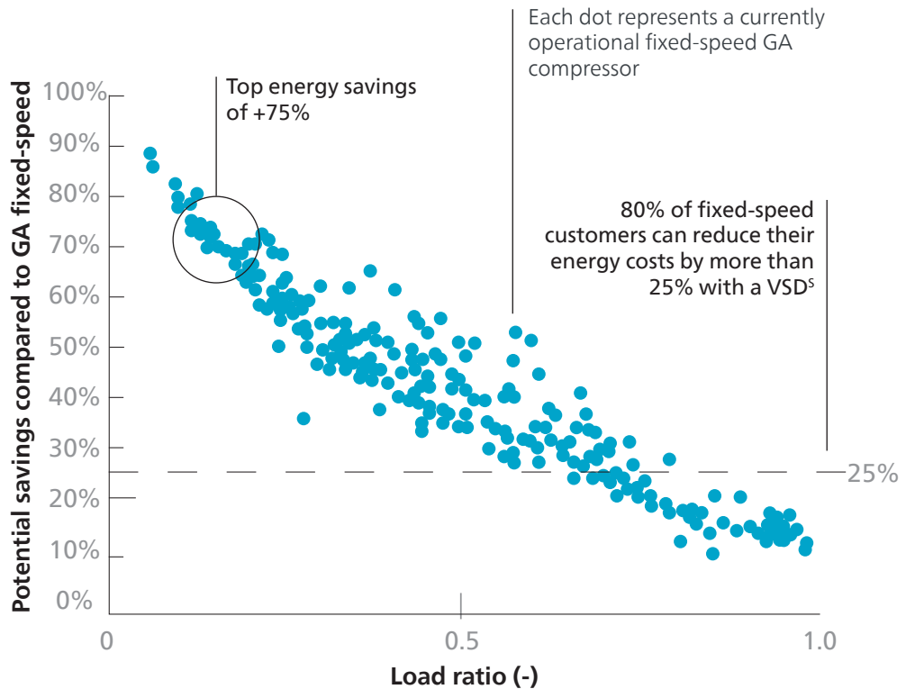
Potential savings compared to GA fixed-speed 22 kW, 7 bar example based on real customer data
